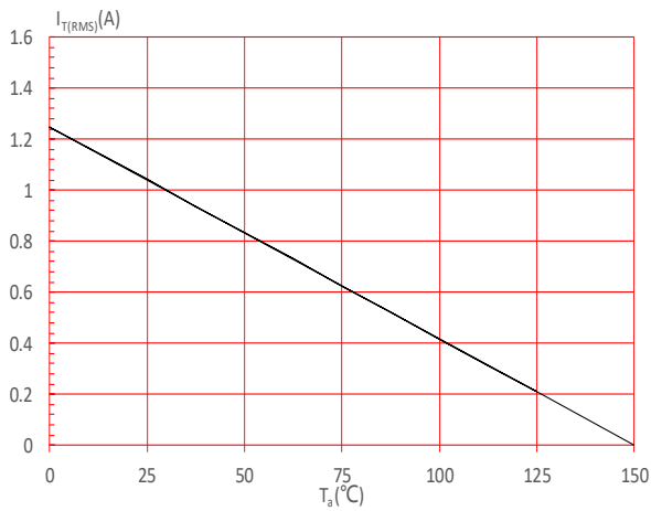
FIG.5: On-state characteristics
