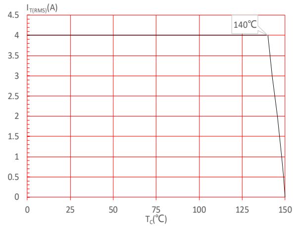
FIG.4: On-state characteristics
