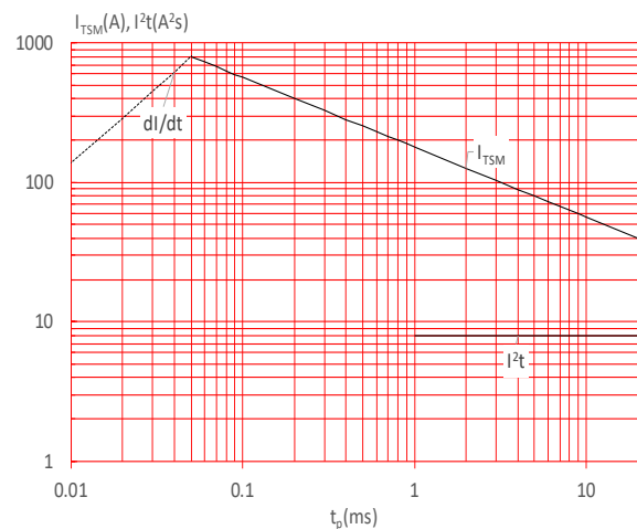
FIG.6: Non-repetitive surge peak on-state current for a sinusoidal pulse with width t_p < 20ms , and corresponding value of I^2t ( di/dt < 80A/\mu s )
