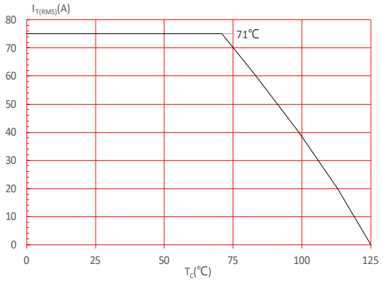
FIG.4: On-state characteristics
