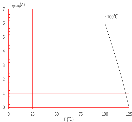
FIG.4: On-state characteristics
