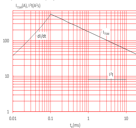
FIG.6: Non-repetitive surge peak on-state current for a sinusoidal pulse with width t_p < 20ms , and corresponding value of I^2t ( di/dt < 50A/μs )
