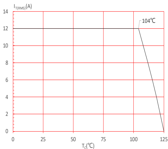
FIG.4: On-state characteristics
