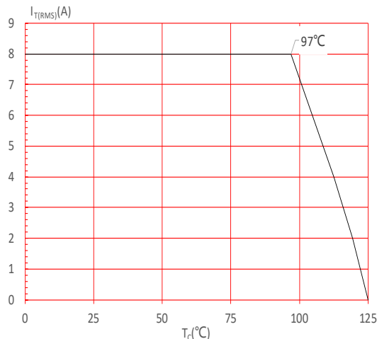
FIG.4: On-state characteristics
