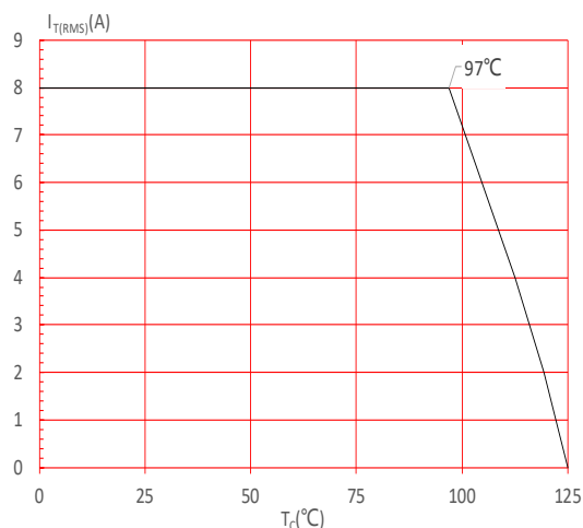
FIG.4: On-state characteristics
