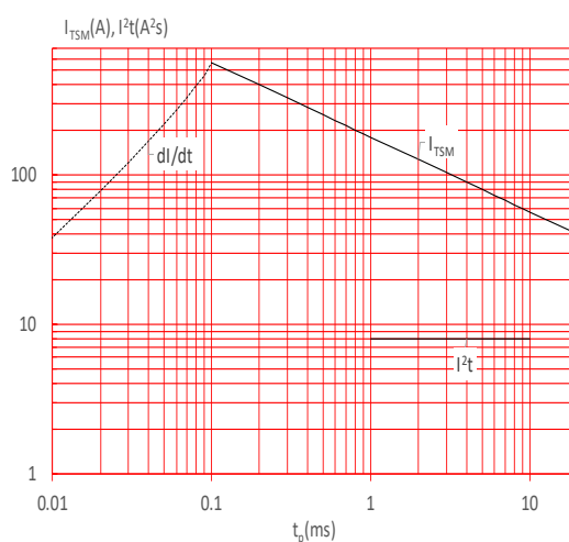
FIG.6: Non-repetitive surge peak on-state current for a sinusoidal pulse with width t_p < 20ms , and corresponding value of I^2t ( di/dt < 50A/\mu s )
