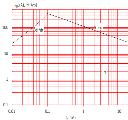
FIG.6: Non-repetitive surge peak on-state current for a sinusoidal pulse with width t_p < 20ms , and corresponding value of I^2t ( di/dt < 100A/\mu s )
